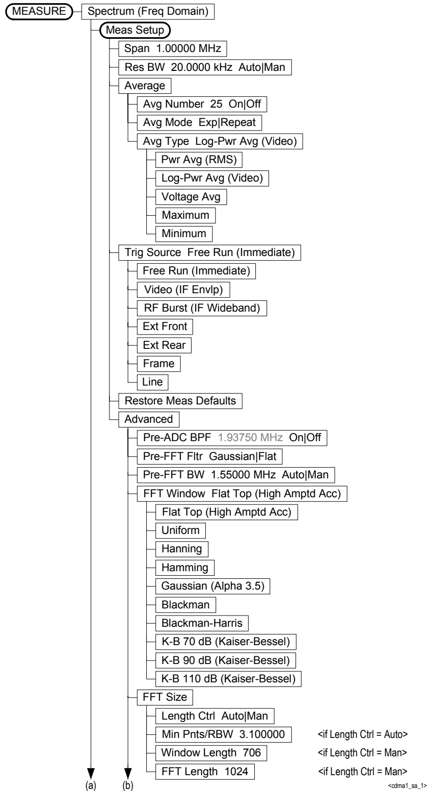
Figure 6-9 Spectrum (Freq Domain) Measurement Key Flow (1 of 3)
