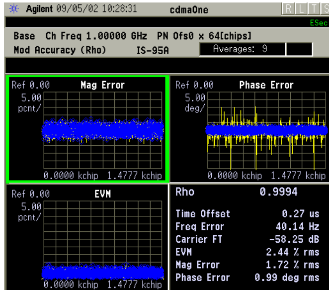
Figure 2-12 Modulation Accuracy Result - I/Q Error View (chip dots on)
