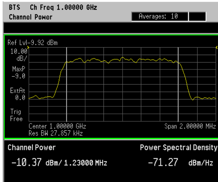
Figure 2-9 Channel Power Measurement Result
